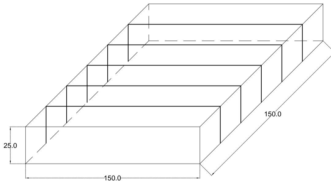
ISOMETRIC VIEW
